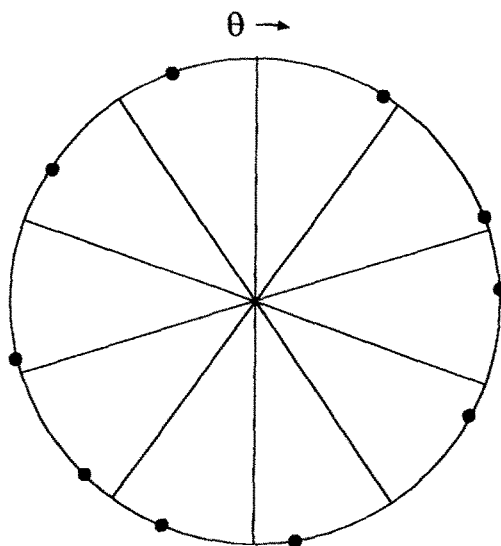
Fig. 9.2. Division of the circle by the point generated by \text{mod}_{2\pi}(2\pi m/\tau^k) (for k = 1 and m = 1, 2, 3, \dots, 10 ). The origin is marked by \theta = 0 and the direction of increasing \theta is shown by the arrow. The radial lines divide the circle into ten equal segments in order to better illustrate the distribution of points on the circumference.
