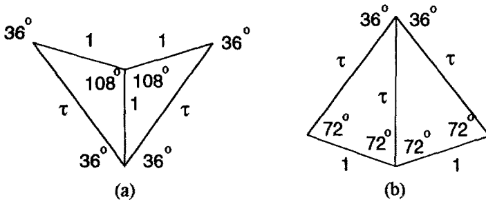
Fig. 11.9. Dissection of darts and kites, (a) and (b), respectively, into golden triangles. Angular and length relationships are illustrated.
