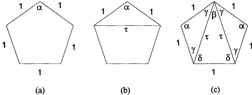
Fig. 3.1. (a) The regular pentagon with an edge length of 1, (b) the regular pentagon showing the diagonal of length \tau and (c) the regular pentagon dissected into two golden triangles and a golden gnomon.
