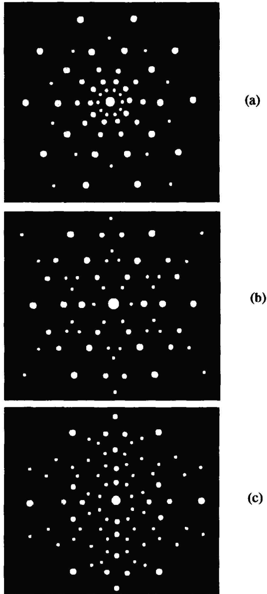
Fig. 12.9. Electron diffraction patterns of the icosahedral quasicrystal Al_{65}Cu_{20}Fe_{15} showing (a) fivefold symmetry axis, (b) threefold symmetry axis and (c) twofold symmetry axis.
