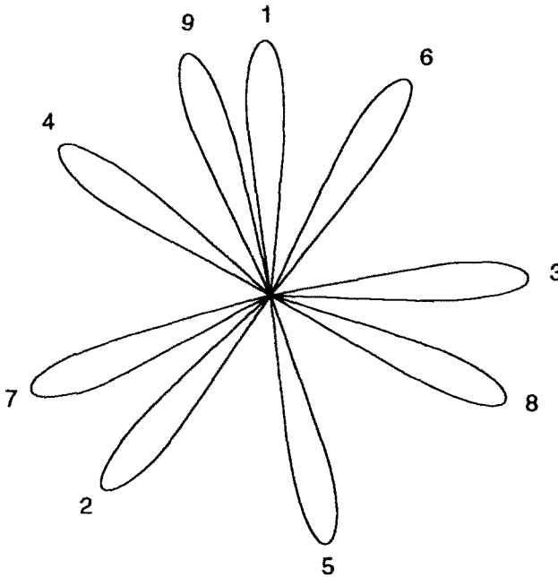
Fig. 13.6. Optimal spacing of leaves on a stem with a growth angle of 2\pi\tau (radians). The numbers indicate the order of growth.
