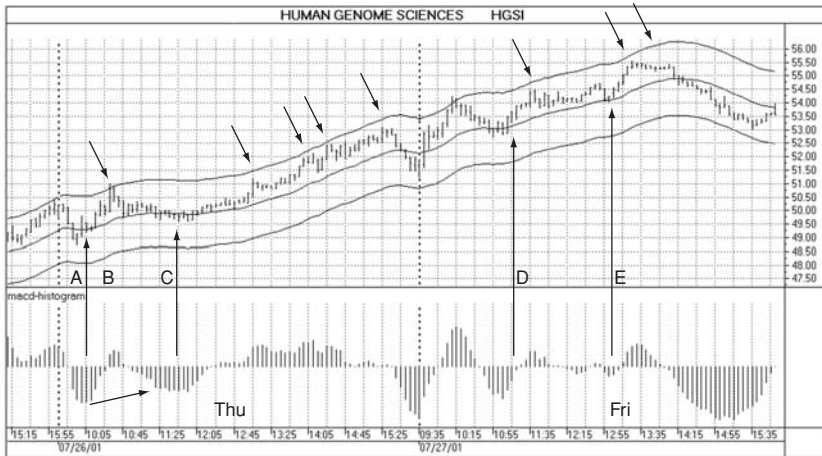
Figure 6.4 Day-Trading—Five-Minute Chart
