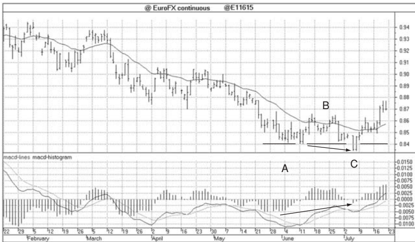
Figure 5.9 MACD-Histogram
