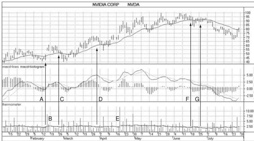
Figure 6.7 Market Thermometer
