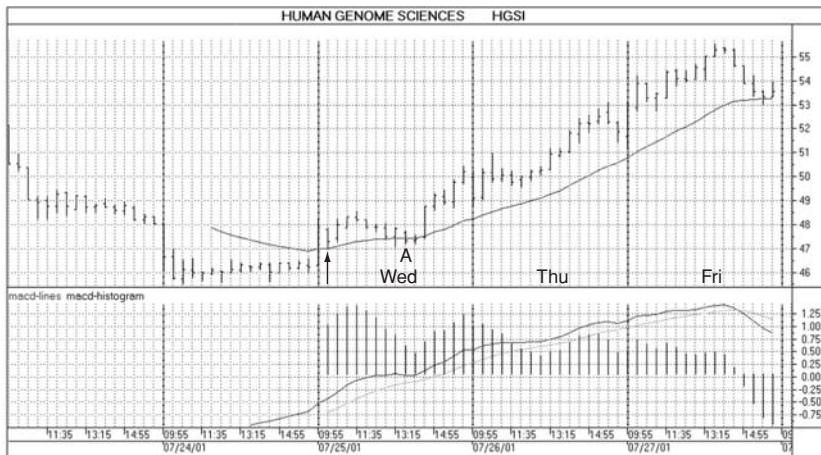
Figure 6.3 Day-Trading—25-Minute Chart
