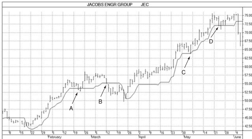
Figure 6.8 SafeZone Stops—Uptrend
