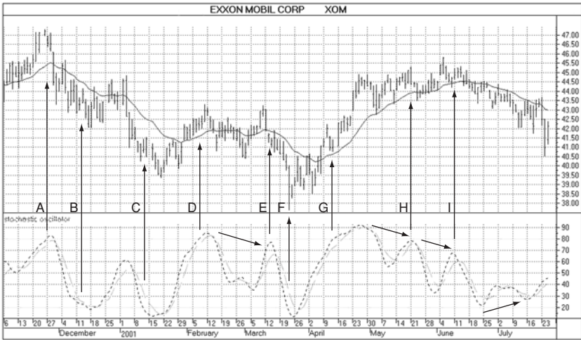
Figure 5.14 Stochastic
