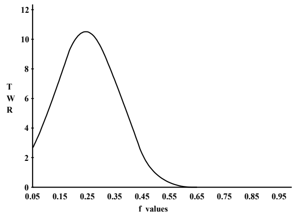
Figure 1-1 20 sequences of +2, -1.
