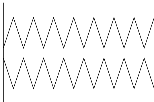
Figure 1-3 Negative correlation ( r = -1.00 ).
