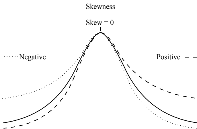
Figure 3-2 Skewness
