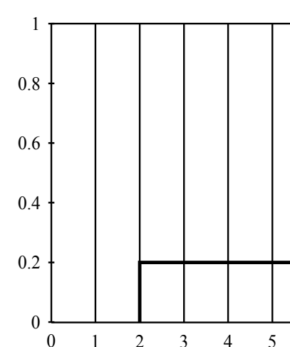
Figure B-1 Probability density functions for the Uniform Distribution ( A = 2, B = 7 ).
