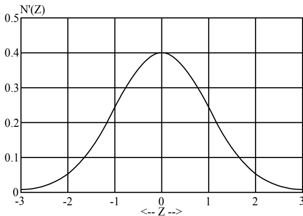
Figure 3-7 The Normal Probability density function.
