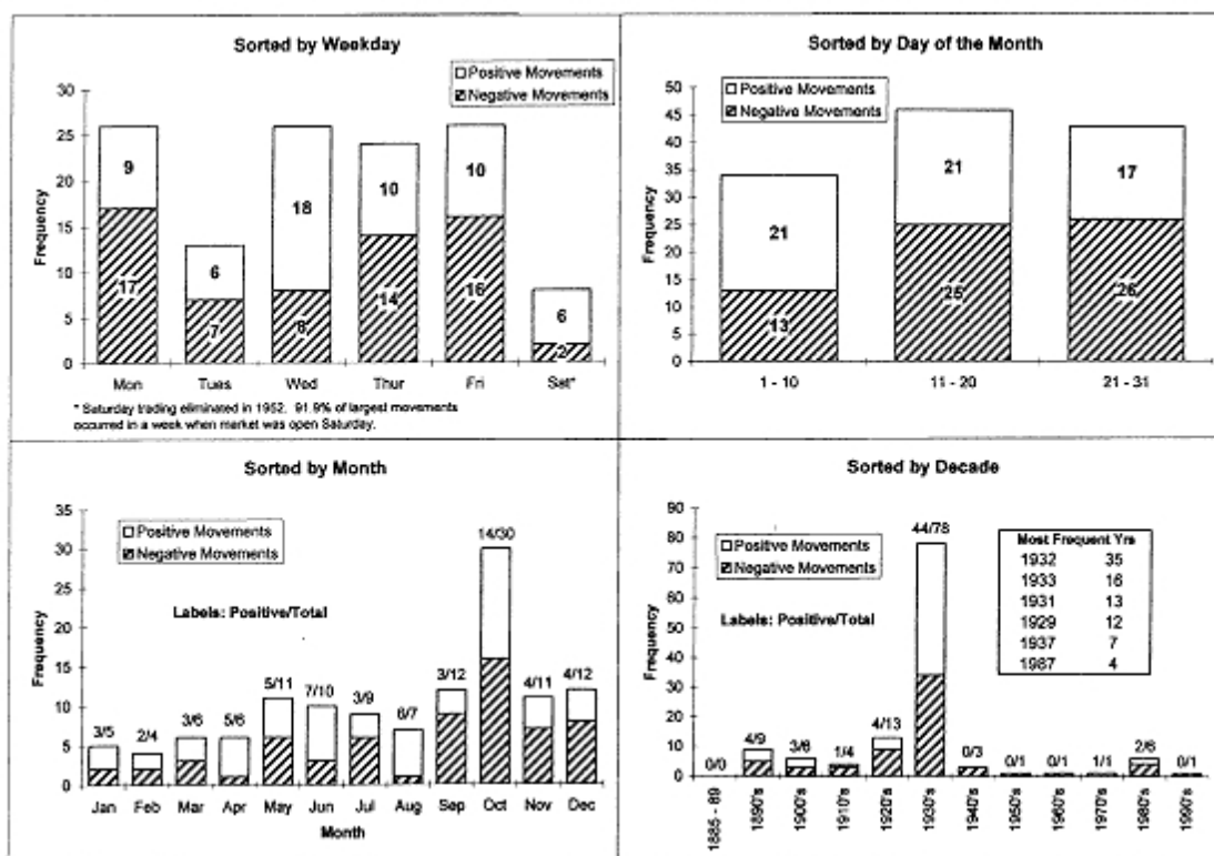
FIGURE 16-4 Distribution of Dow Industrial Changes over 5 Percent, 1885-1997
