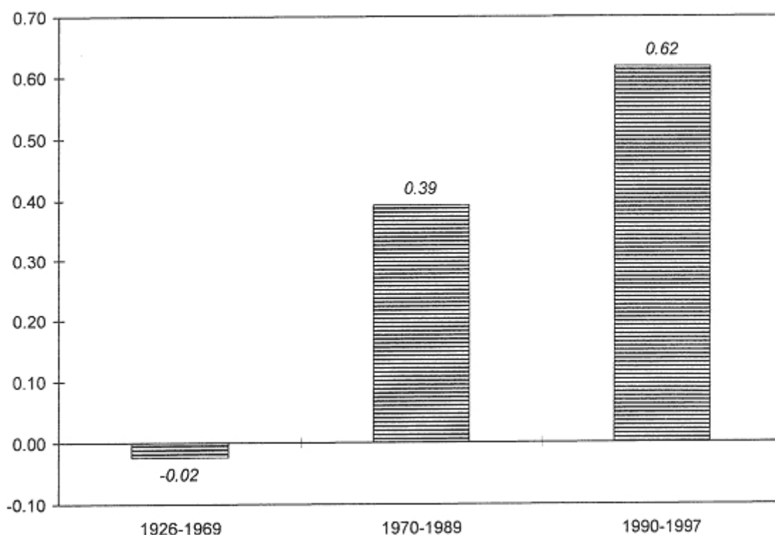
FIGURE 2-5 Correlation Coefficient Between Annual Stock and Bond Returns
